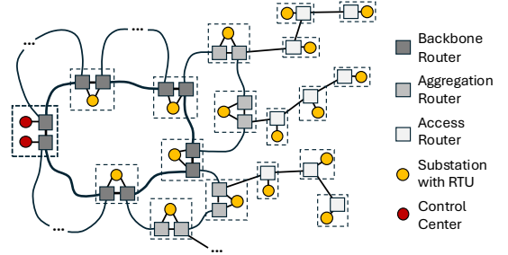
Fig. 2: Hierarchical communication network topology abstracted from the real-world structure of a German DSO.
