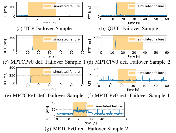
Fig. 6: RTTs before, during, and after emulating an outage of the main connection (marked in orange).
